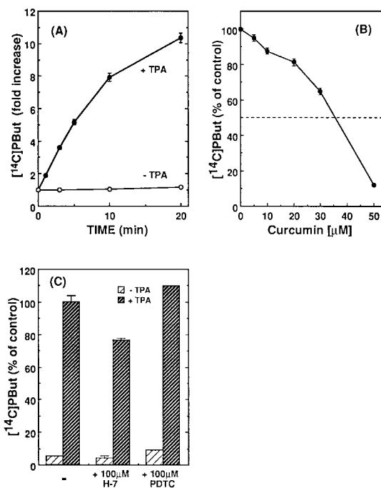
Fig. 2. TPA-induced PLD activation. A: [ ^{14} C]palmitate-labeled J774.1 cells were stimulated with 100 nM TPA (closed circle) in the presence of 1% butanol. The level of [ ^{14} C]PBut in the absence of TPA at 0 min was taken as 1. B: Dose-dependent effect of curcumin on PLD activity. [ ^{14} C]Palmitate-labeled J774.1 cells were incubated with various concentrations of curcumin at 37°C for 30 min, then stimulated with 100 nM TPA at 37°C for 20 min. The level of [ ^{14} C]PBut in the presence of TPA without curcumin was taken as 100%. C: [ ^{14} C]Palmitate-labeled J774.1 cells were incubated with or without 100 \mu M H-7 and 100 \mu M PDTC at 37°C for 30 min, then stimulated with 100 nM TPA at 37°C for 20 min. The level of [ ^{14} C]PBut in the presence of TPA without drugs was taken as 100%. The data shown are mean values \pm S.D. of three independent experiments.
